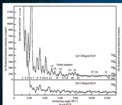
Neutron scattering by collagen
